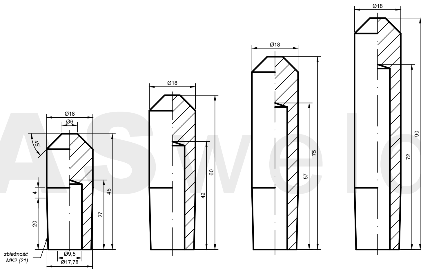
AW: B1(6)-18.45-21*
