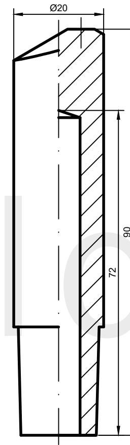
AW: D(6)-20.90-21*
