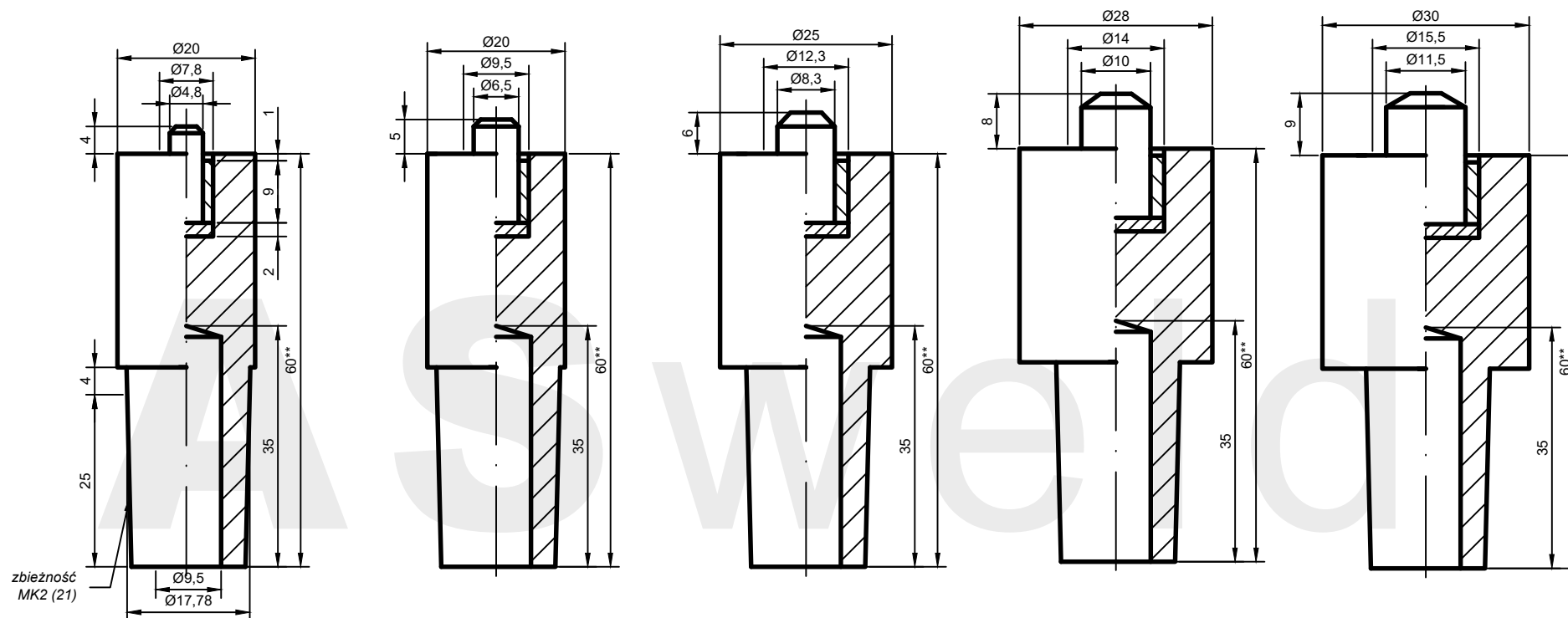
AW: M12N-28.60-21*
