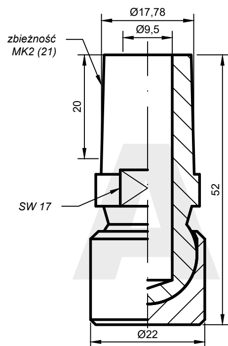
AW: PK19-22.52-21*
