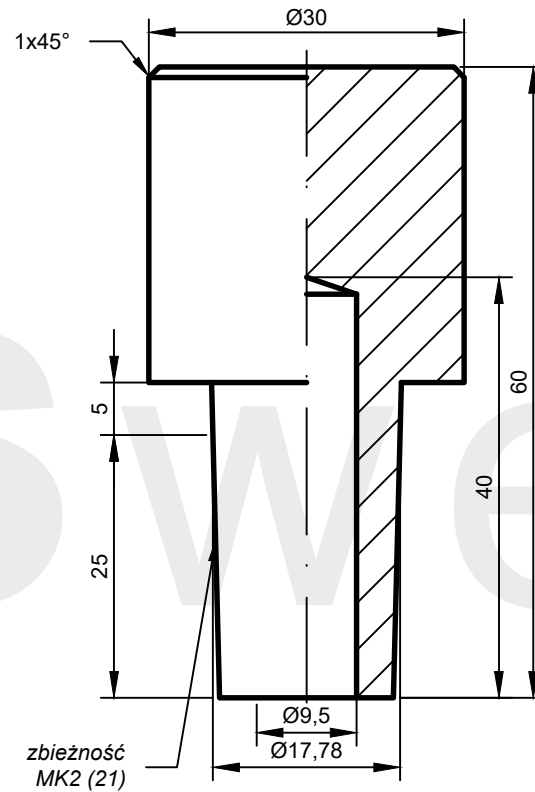
AW: C-30.60-21
