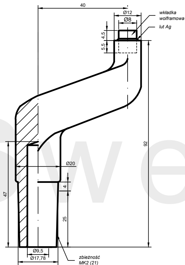
AW: W8-F03-21
