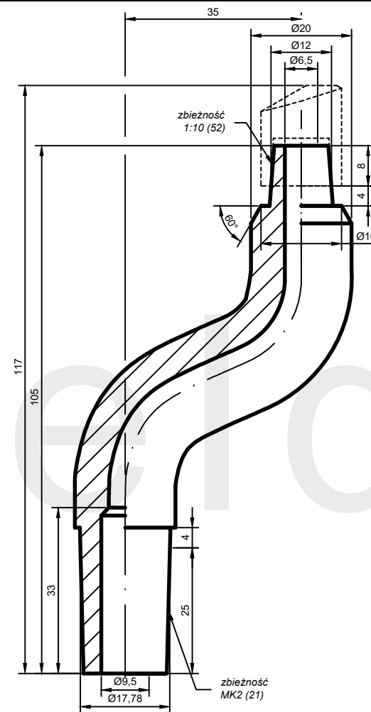
AW: TR52-20.105.35-21*
