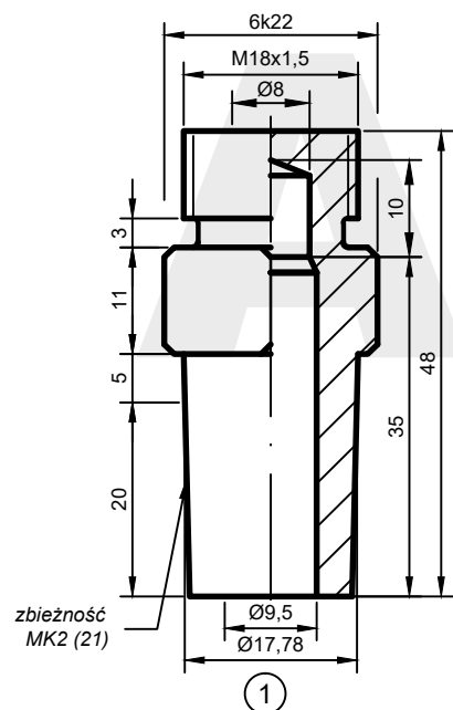
AW: TR-6k22.48-21/18M1,5
