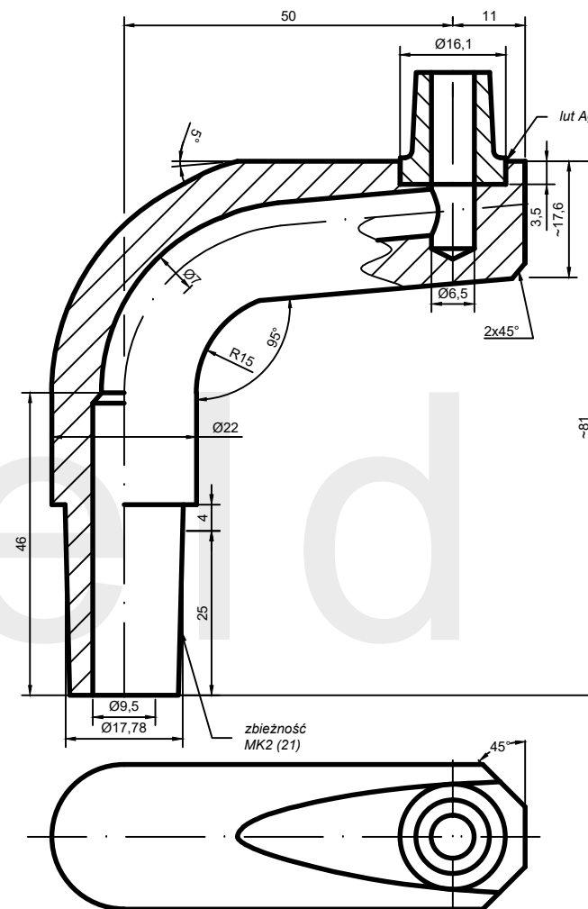
AW: TR52-22.81.50-21*
