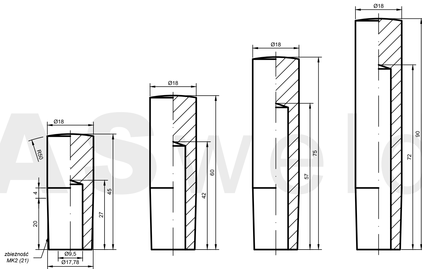
AW: A(50)-18.45-21*
