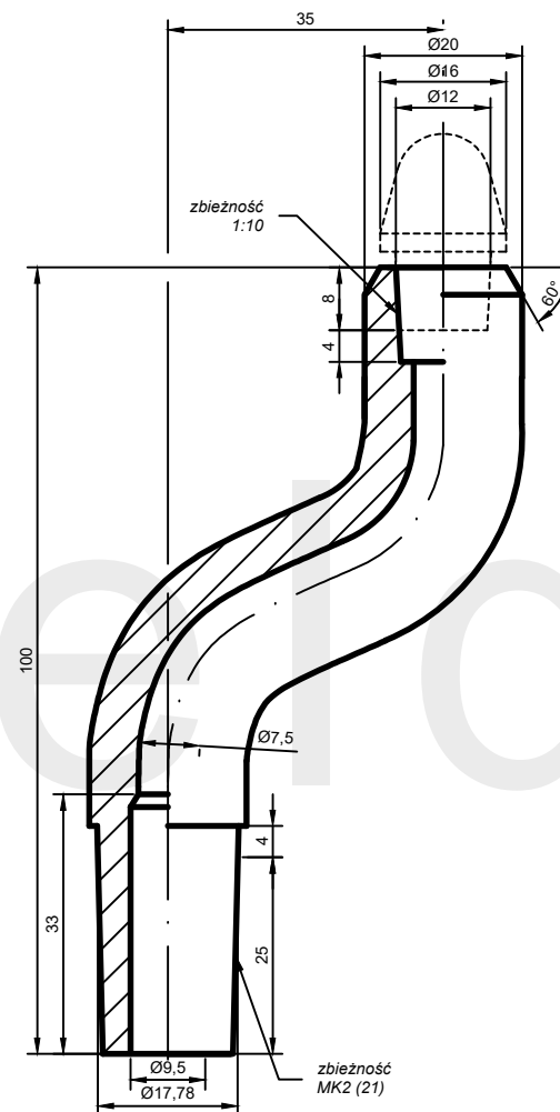
AW: GN40-20.100.35-21
