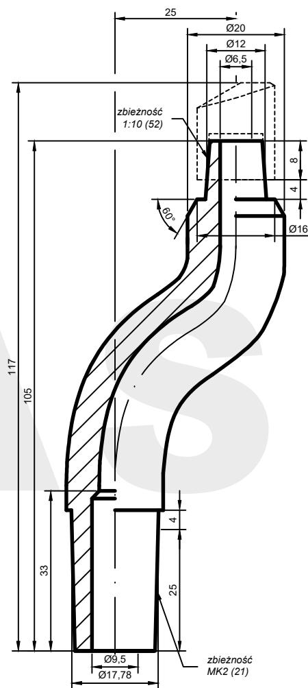
AW: TR52-20.105.25-21*
