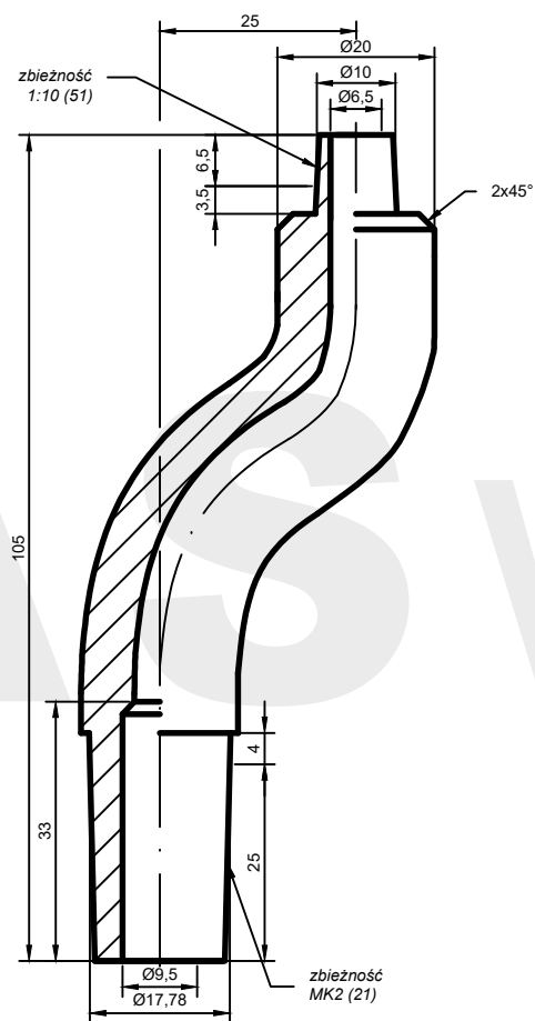
AW: TR51-20.105.25-21*
