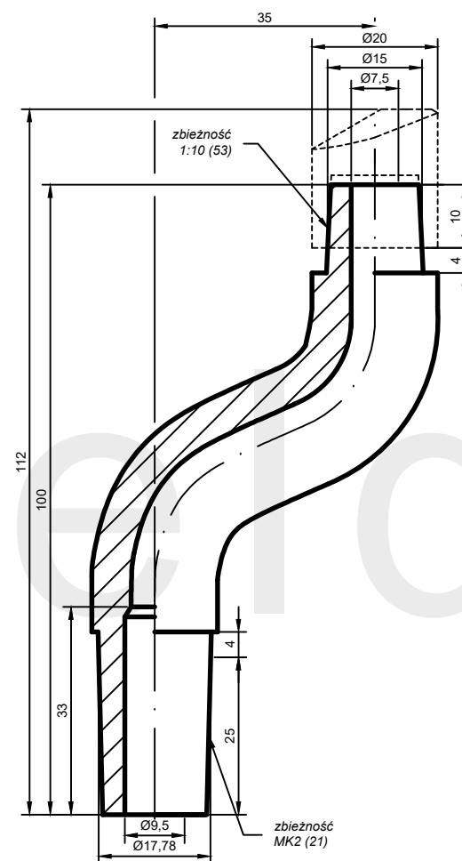
AW: TR53-20.100.35-21*
