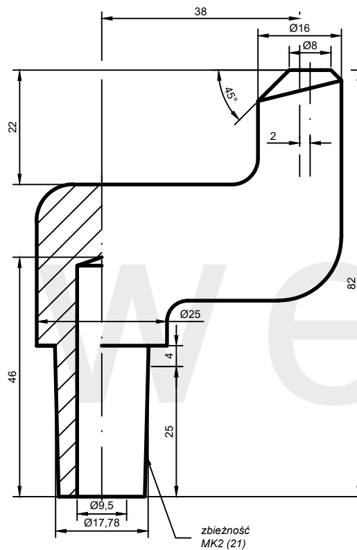
AW: F11(8)-25.82.38-21
