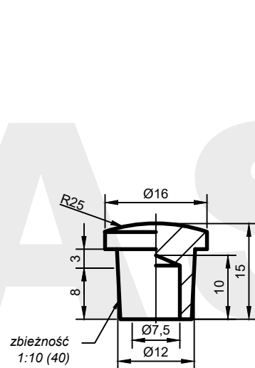
AW: A(25)-16.15-40
