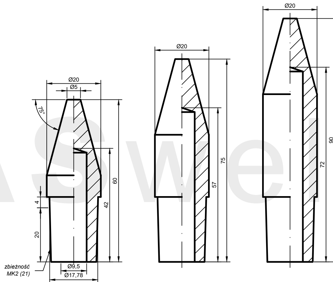
AW: B3(5)-20.60-21
