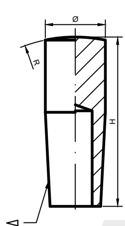
AW: A(R)-Ø.H- ▽
