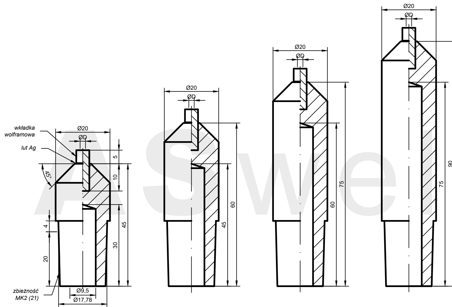
AW: WØD-20.45-21*
