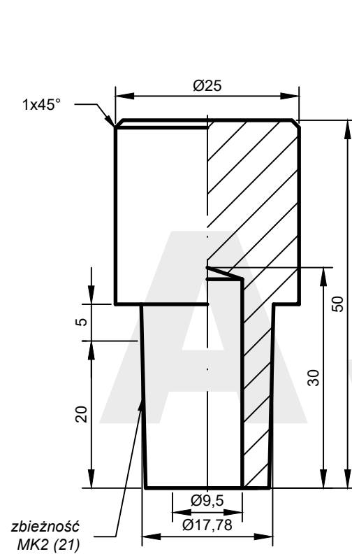
AW: C-25.50-21
