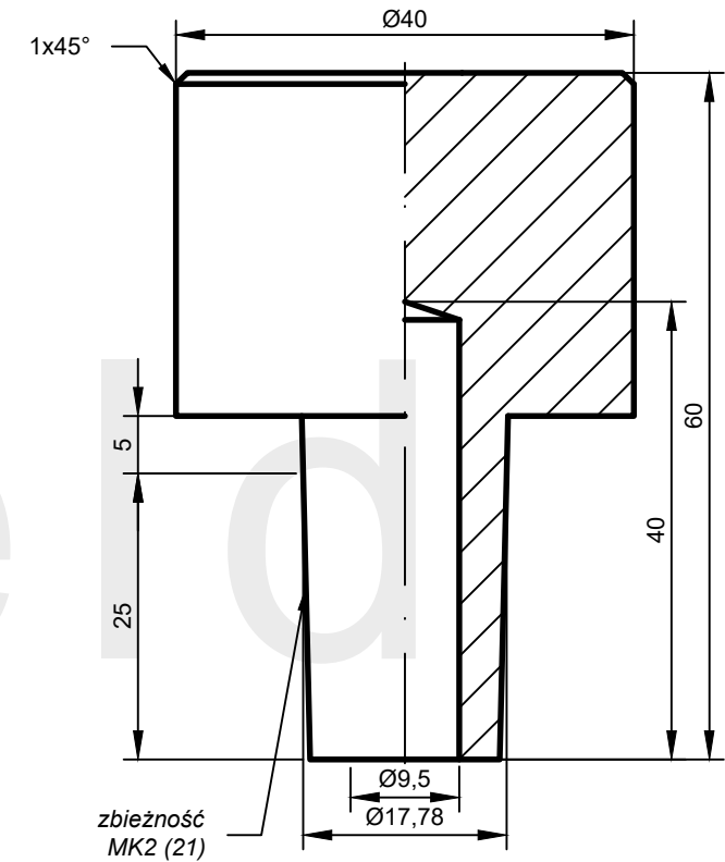
AW: C-40.60-21*
