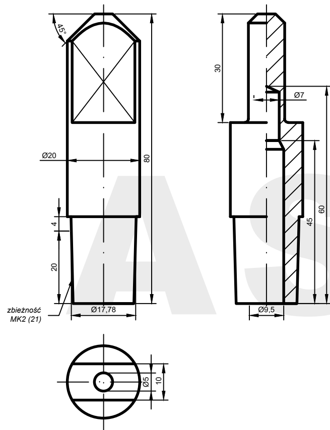
AW: B1(5)-20(20x10).80-21*
