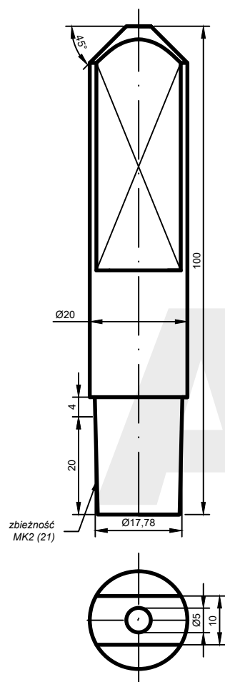
AW: B1(5)-20(20x10).100-21*
