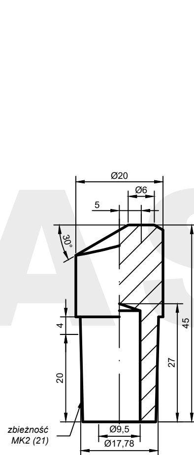
AW: D(6)-20.45-21*
