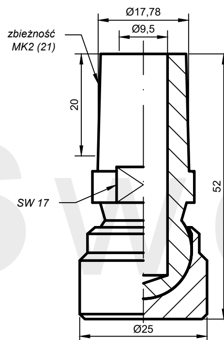
AW: PK19-25.52-21
