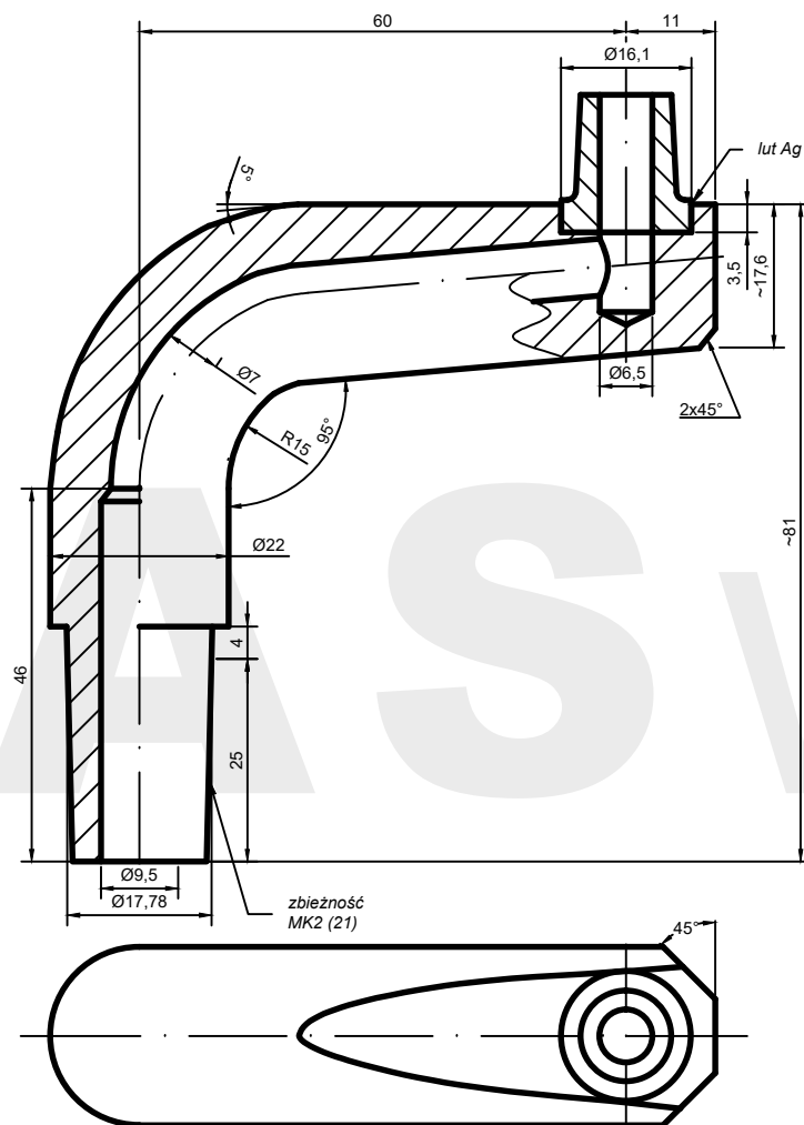
AW: TR52-22.81.60-21*
