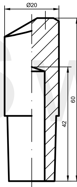
AW: D(6)-20.60-21
